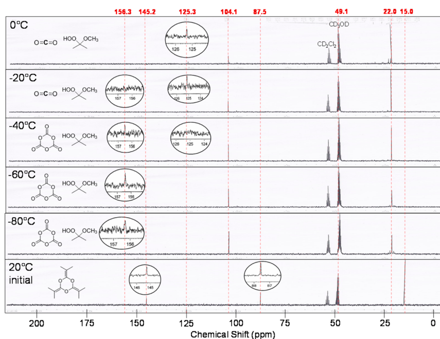
Figure 1. 13 C NMR spectra from the triolefin-trione–ozone reaction. The lowest spectrum is the substrate 2a CD 2 Cl 2 /CD 3 OD solution prior to ozone treatment. The series spectra above were recorded after the -78 °C ozone saturation and purging from this solution at successive 20 °C temperature increments from -80 to 0 °C. The compound structures for which resonances are assigned are depicted at the left of each spectra and the chemical shifts discussed in the text are indicated by the dashed lines and values at the top of this figure. Those resonances of particular importance have a magnified insert.
